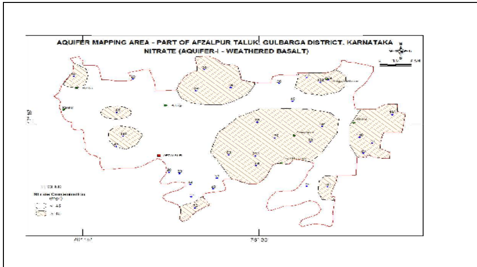
Fig 3.3: Concentration of Nitrate (Aquifer-I)
